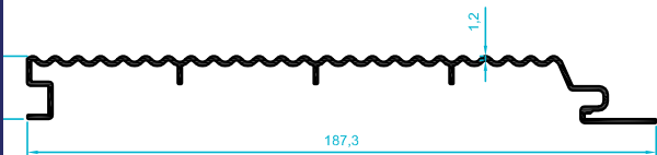
207.09 1,391 kg/m
