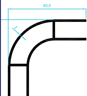
701.43 1,585 kg/m
