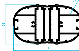
207.123 2,382 kg/m
