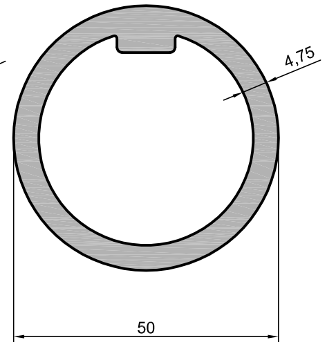
204.31 1,943 kg/m
