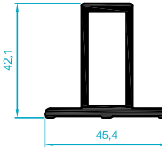
326.39 1,009 kg/m
