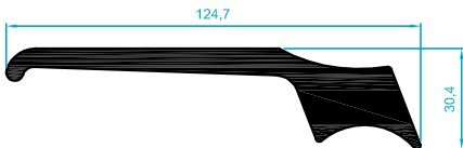
326.48 3,235 kg/m
