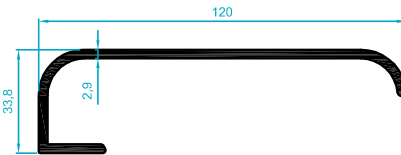
326.43 1,335 kg/m
